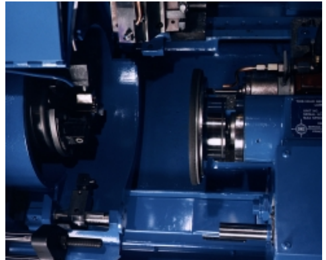
Slide Bar Arrangement on a 1SN-2XC. Photograph shows proximity of independent facing and bore grinding wheels, and position of each single-point dressing diamond. The fore-most device (lower left) is the servo-motor-controlled face feeding stop.
